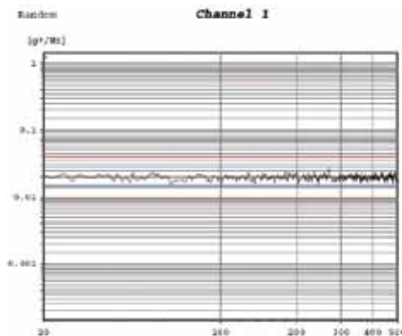
Sample random vibration profile at 3.1GRMS, Y Axis
